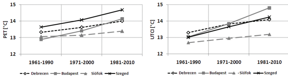
Fig. 2 Variation of 30-year averages of annual means of Physiologically Equivalent Temperature (left) and Universal Thermal Climate Index (right) at 12 UTC
