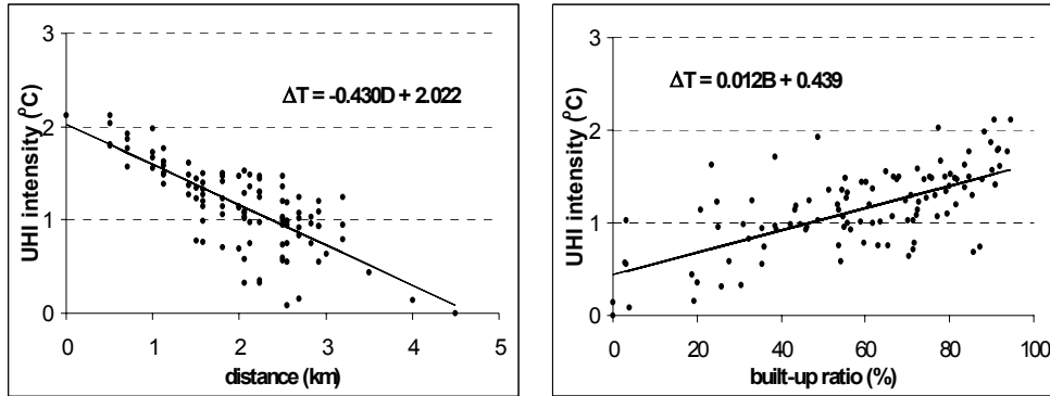
Fig. 4 Maximum UHI intensity ( \Delta T ) as a function of the distance from the centre ( D ) and built-up ratio ( B ) with the best fit regression lines in the heating season (16 October - 15 April) in Szeged
