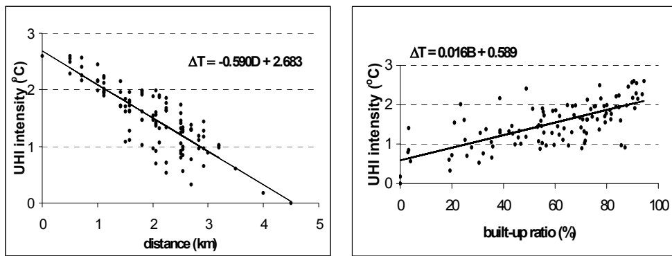
Fig. 2 Maximum UHI intensity ( \Delta T ) as a function of the distance from the centre ( D ) and built-up ratio ( B ) with the best fit regression lines in the one-year period (March 1999 - February 2000) in Szeged
