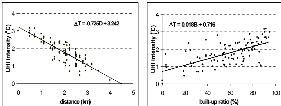
Fig. 3 Maximum UHI intensity ( \Delta T ) as a function of the distance from the centre ( D ) and built-up ratio ( B ) with the best fit regression lines in the non-heating season (16 April - 15 October) in Szeged
