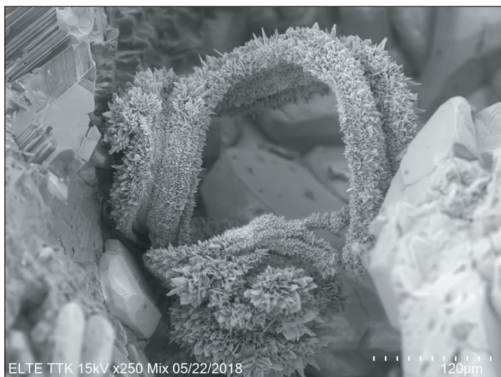
▲ Fig. 3.92b Silver, wiry aggr. with acanthite thorns on their surfaces, Vilmos; GK, SEM [DSz]
